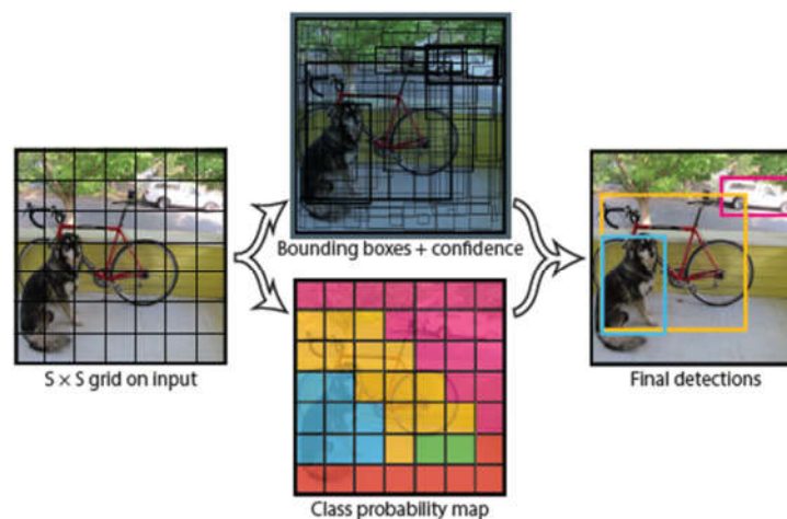
Fig. 8 YOLO object detection procedure
